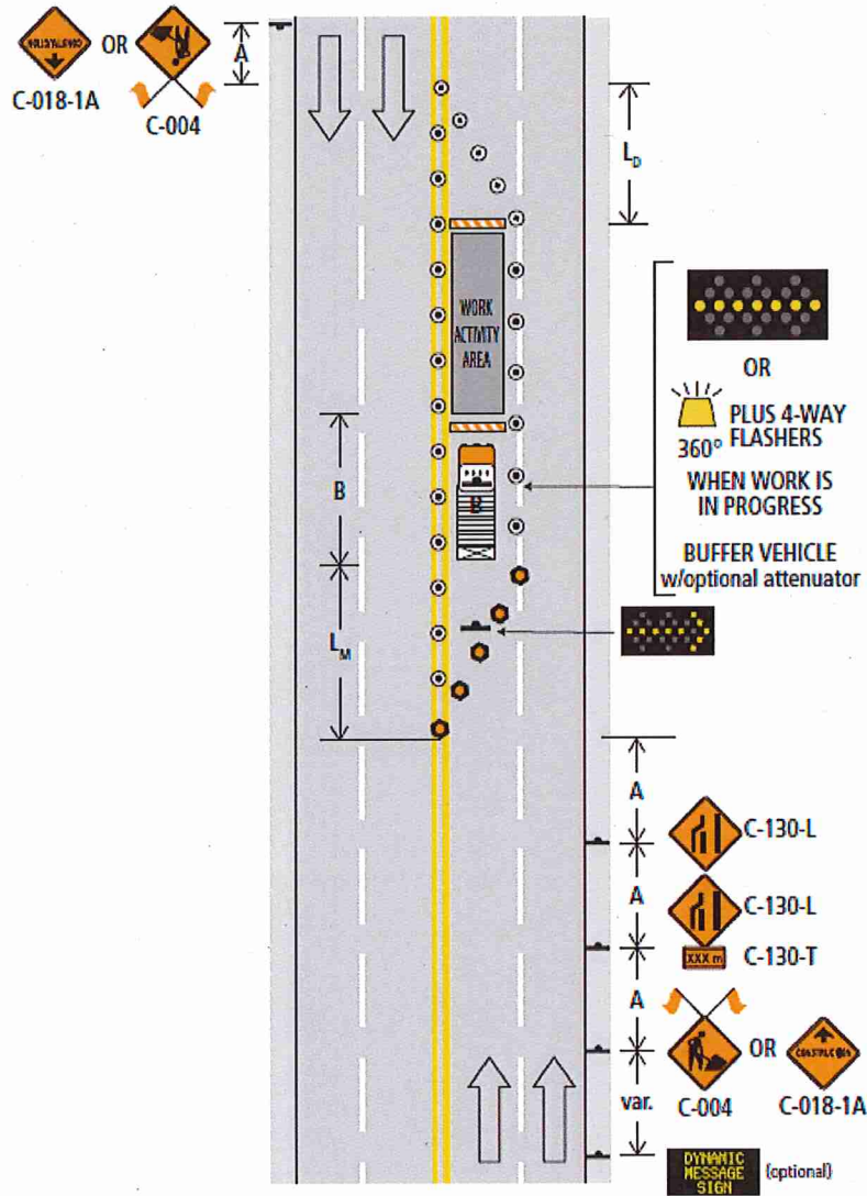
Figure 8.7: Left Lane Closed – Short and Long Duration
